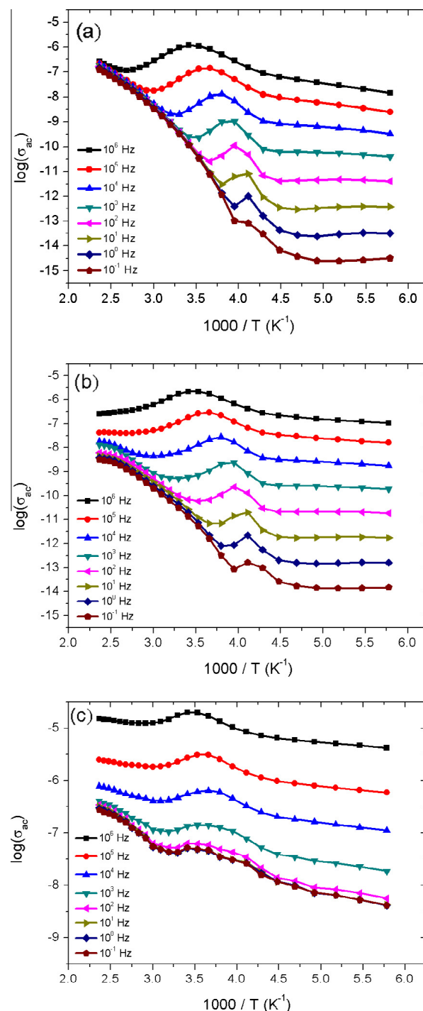
Fig. 8. Conductivity as a function of reciprocal temperature at various frequencies for (a) HNBR, (b) HNBR + 10phr MWCNT and (c) HNBR + 20phr MWCNT systems.
