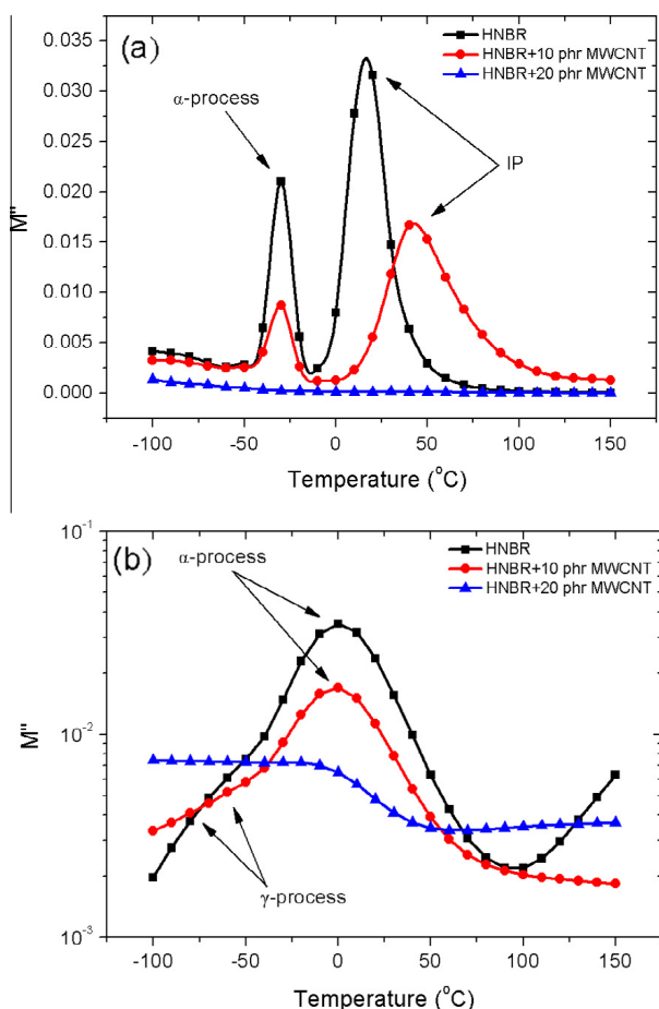
Fig. 7. Variation of modulus loss index with temperature for all studied systems at (a) 10 Hz and (b) 1 MHz.
