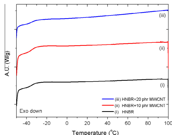
Fig. 3. DSC thermographs of all studied systems.
