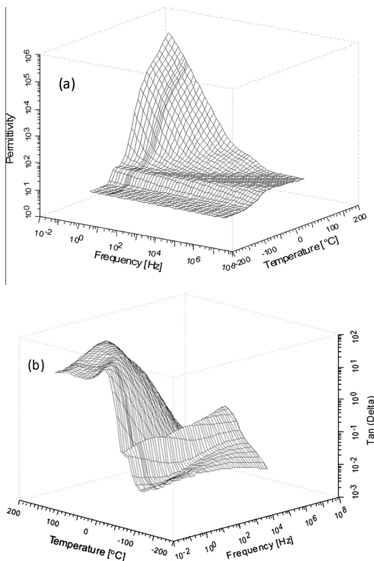
Fig. 4. Variation of (a) real part of permittivity and (b) loss tangent, with temperature and frequency for unfilled HNBR.
