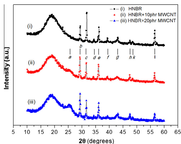
Fig. 2. XRD diffractograms of the (i) HNBR, (ii) HNBR + 10phr MWCNT and (iii) HNBR + 20phr MWCNT systems. Arrow lines indicate peaks positions for a: graphite-like peak, b, f, h, k: calcite, c, d, e, h, l: ZnO and g: MgO peak.
