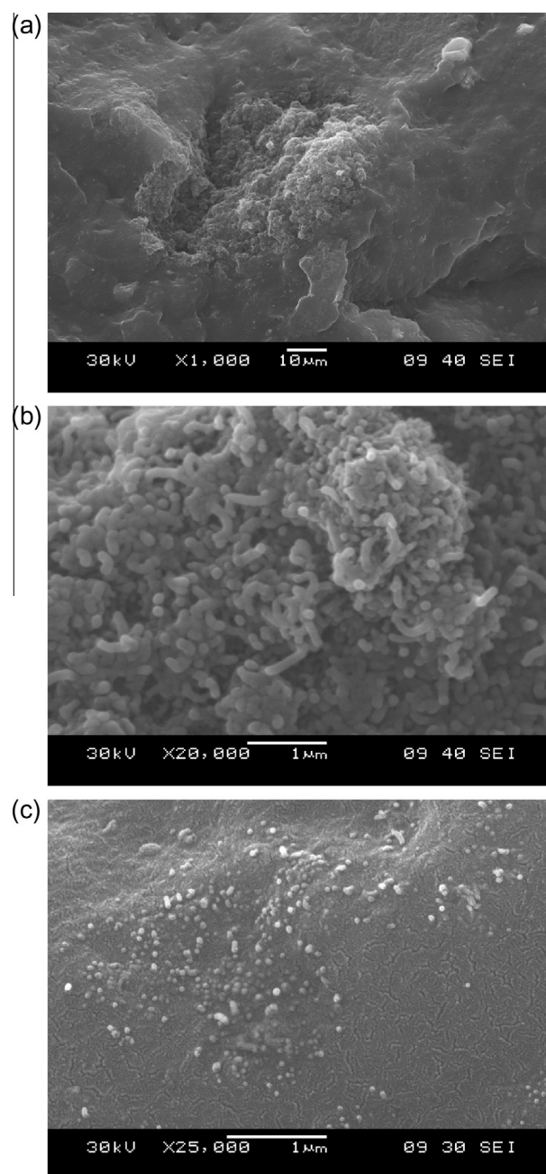
Fig. 1. SEM images from cryofractured surface of the HNBR + 20phr MWCNT specimen at (a) 1000 \times , (b) 20,000 \times and (c) 25,000 \times magnification.
