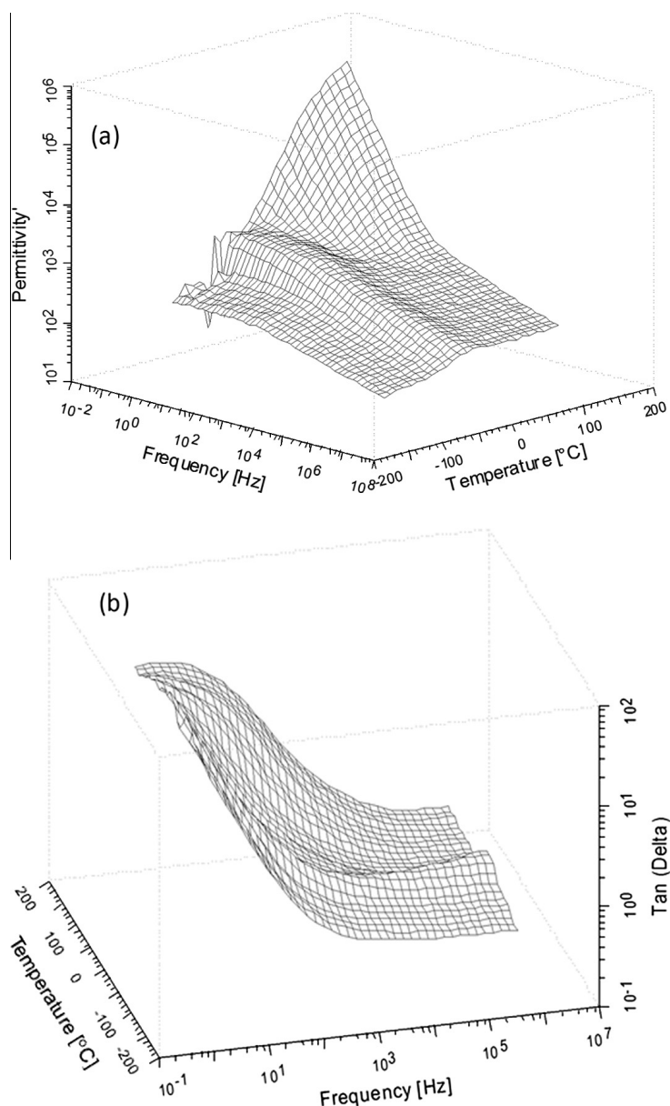
Fig. 6. Variation of (a) real part of permittivity and (b) loss tangent, with temperature and frequency for the HNBR + 20phr MWCNT system.
