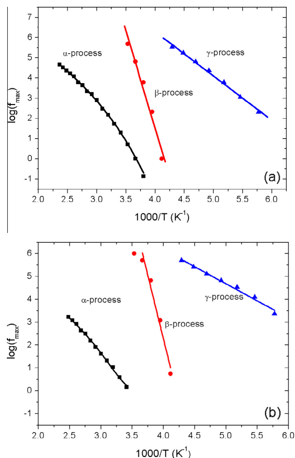
Fig. 9. Loss peak position, of the recorded relaxations, as a function of reciprocal temperature for (a) HNBR and (b) HNBR + 10phr MWCNT systems.
