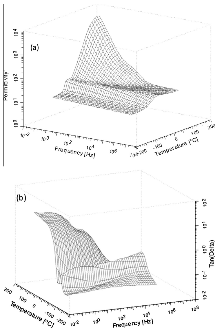
Fig. 5. Variation of (a) real part of permittivity and (b) loss tangent, with temperature and frequency for the HNBR + 10phr MWCNT system.
